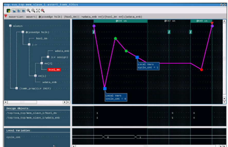
Assertion thread viewer in Visualizer.
