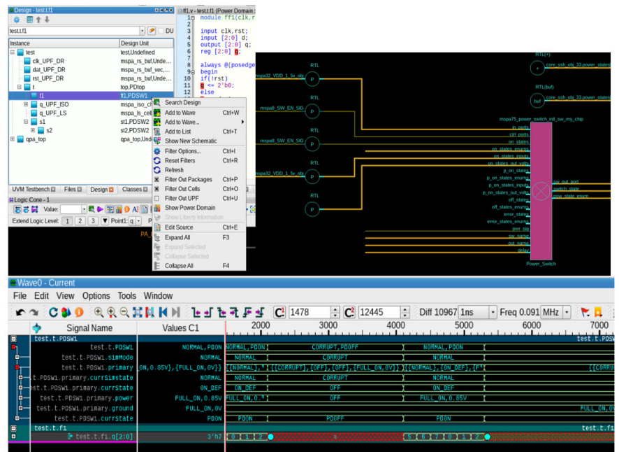
Advanced power-aware debug in Visualizer.
