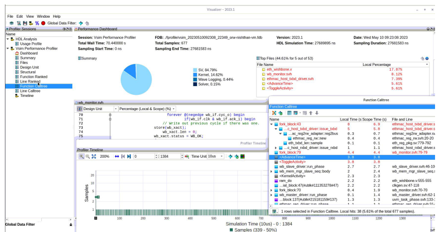
The QuestaSim intuitive performance profiler.
